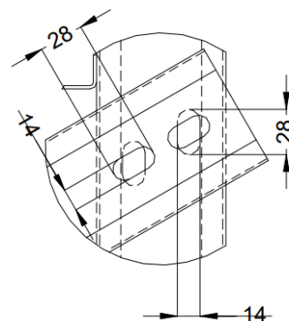
DETAL / DETAIL B SKALA / SCALE 1 : 5
